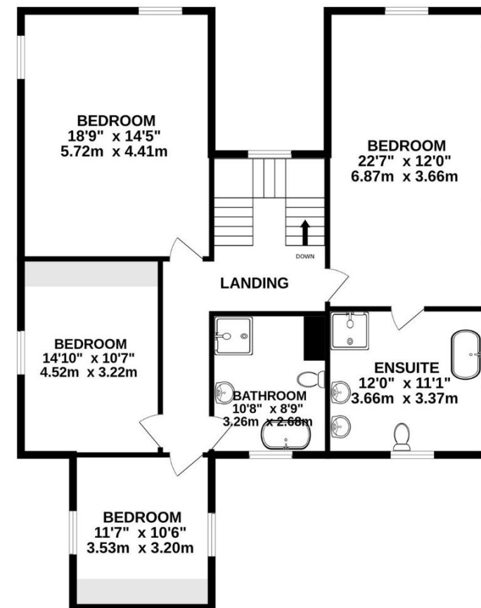
1ST FLOOR 1205 sq.ft. (112.0 sq.m.) approx.
